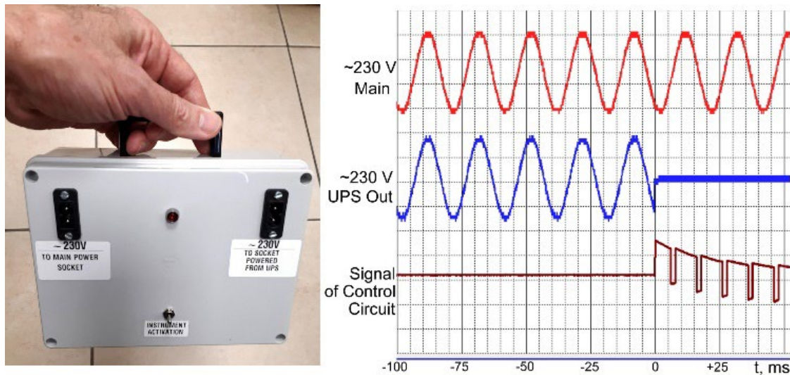
Fig. 25. Simple tester for express verification of the serviceability of the UPS unit after the HEMP impact.
