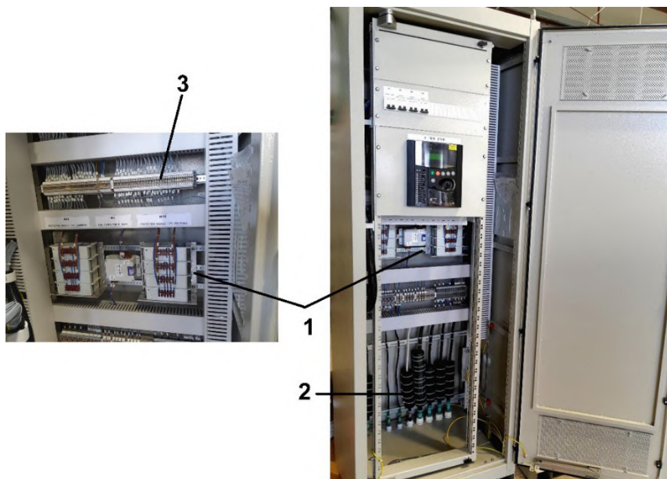
Fig. 17. Complete control cabinet with a microprocessor-based protection relay, filters and DIN-rail surge arresters. 1 - described above filters; 2 – addition filters; 3 – special surge arresters
