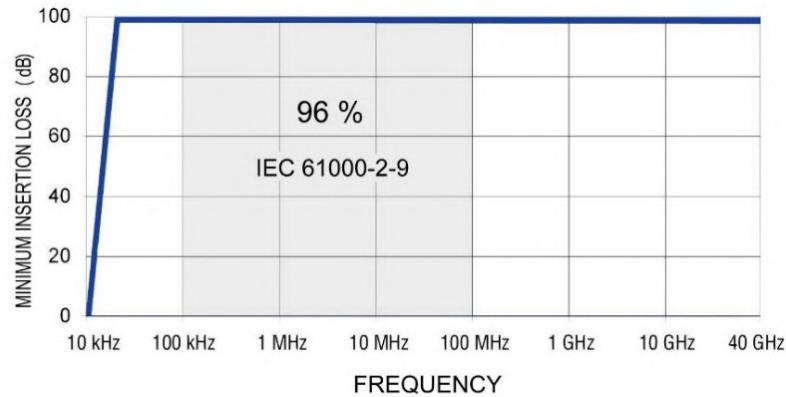
Fig. 5. Typical amplitude and frequency features of HEMP filters represented in ETS-Lindgren's promotional materials.
