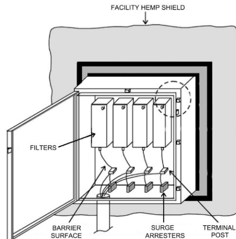
Fig. 9. Design of inlet box for connecting of external cable to a unit protected from HEMP (according to MIL-STD-188-125)
