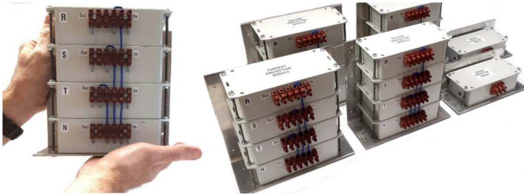
Fig. 15. Special HEMP filters designed by author for installation in current and voltage circuits of microprocessor-based protection relays
