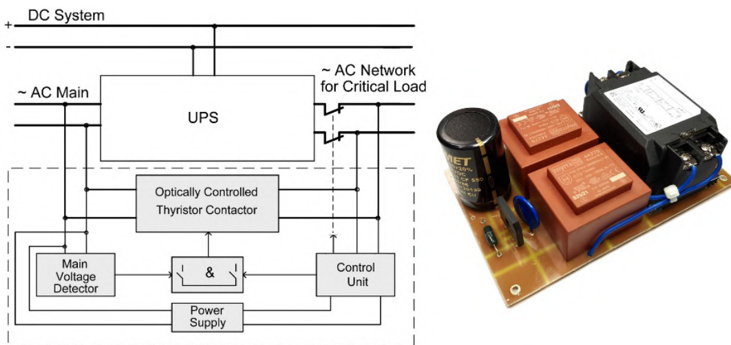
Fig. 24. UPS protection system and its voltage detector
