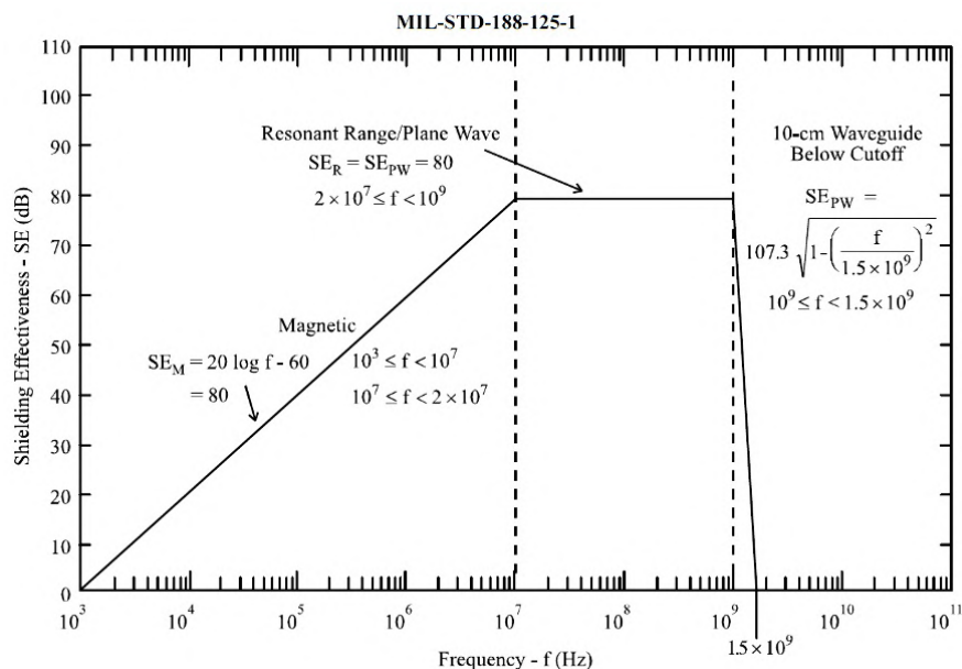
Fig. 4. Minimum HEMP shielding effectiveness requirement according to MIL-STD-188-125-1 [7].
