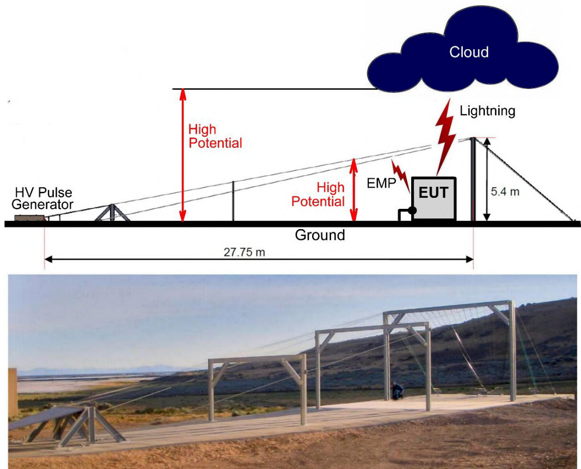
Fig. 11. The antenna system of the test bench simulating HEMP. EUT – equipment under test.
