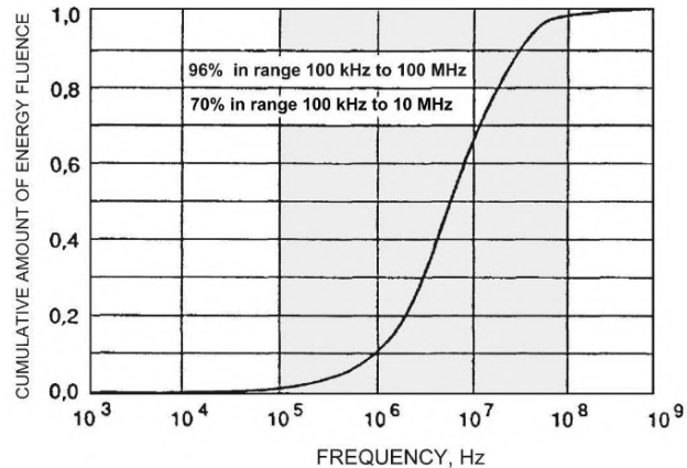
Fig. 7. HEMP energy distribution over the frequency range (see IEC 61000-2-9 [10])
