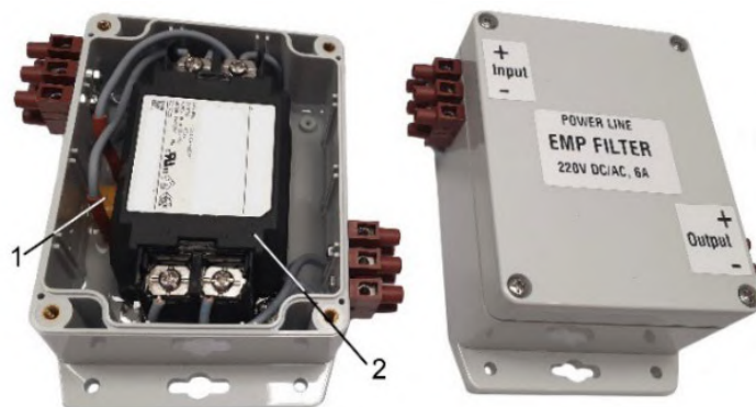
Fig. 16. HEMP power line filter for microprocessor-based protection relays inside the control cabinet. 1 – special high-efficiency surge arrester; 2 – electromagnetic two stage filter.
