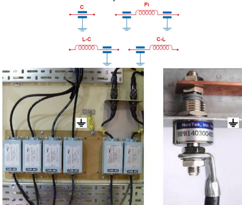
Fig. 8. Simplified design and appearance of various LC-filters against HEMP with parallel capacitive elements that divert impulse energy from the input to the ground
