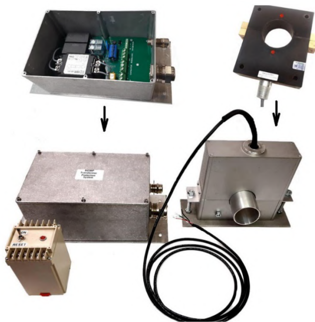
Fig. 18. Simple system for protection of high-power transformer against E3 component of HEMP
