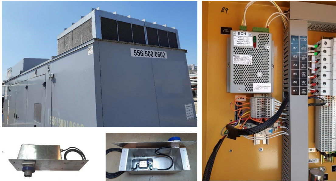
Fig. 28. Protection elements of the backup diesel generator, developed by the author.
