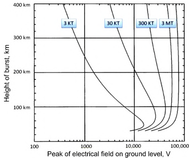
Fig. 13. Variations in the intensity of HEMP exposure.
