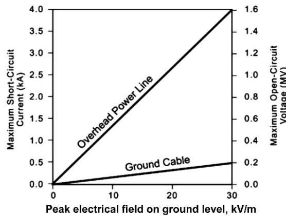
Fig. 14. Voltage and current induced in long overhead lines and ground cables by E1 component of HEMP from kiloton-class yield weapons.
