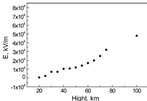
Fig. 12. Changes of the electric field intensity at different HOBs over the explosion center for 1Mt yield [14].
