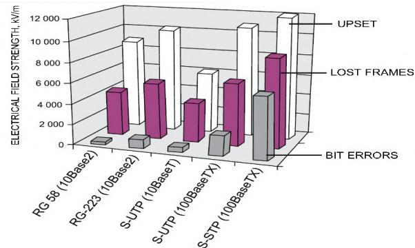
Fig. 3. The level of susceptibility (failures) of the simplest computer network for various network and cables configurations.
