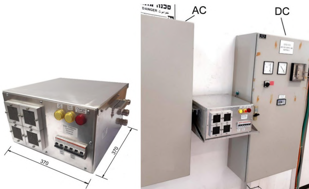
Fig. 20. Automatic HEMP protected charger for auxiliary DC power supply systems of critical infrastructures
