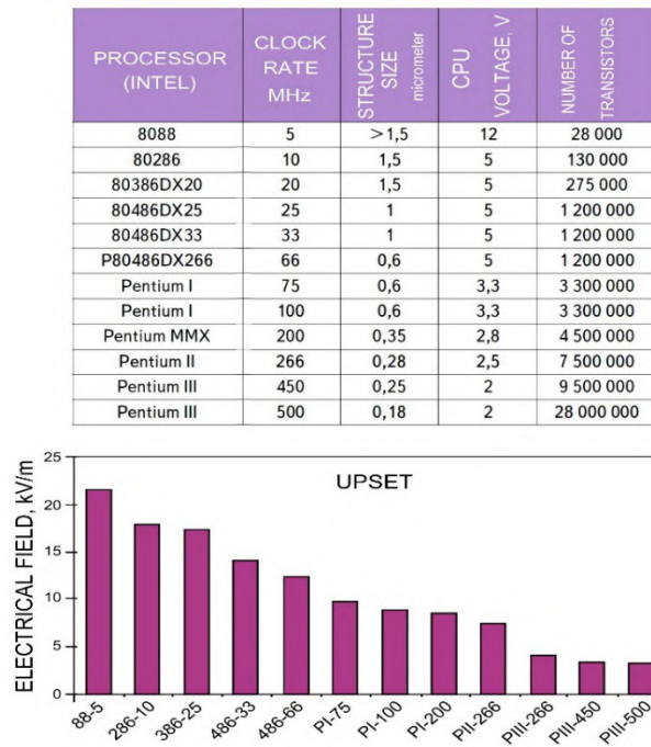
Fig. 2. Information on microprocessors (up to Pentium III inclusive) and the levels of pulse electric field resulting in their malfunctions.
