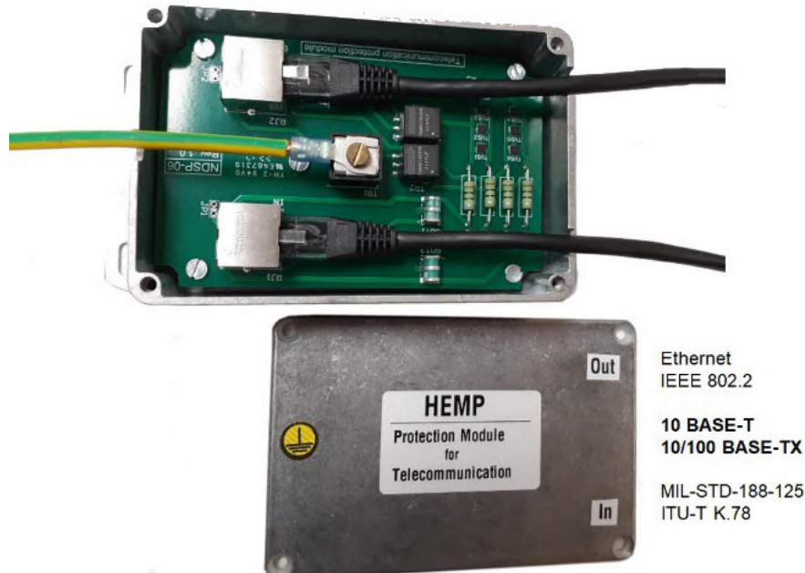
Fig. 23. HEMP protection module for telecommunications
